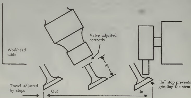
FIGURE 10-15. Valve installed in grinding machine.
